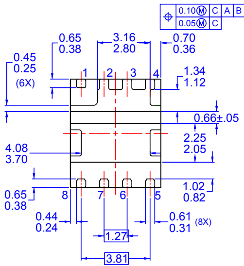
BOTTOM VIEW OPTION - A (SAWN TYPE)
