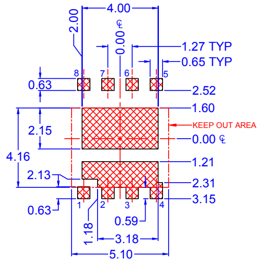
RECOMMENDED LAND PATTERN FOR SAWN / PUNCHED TYPE
