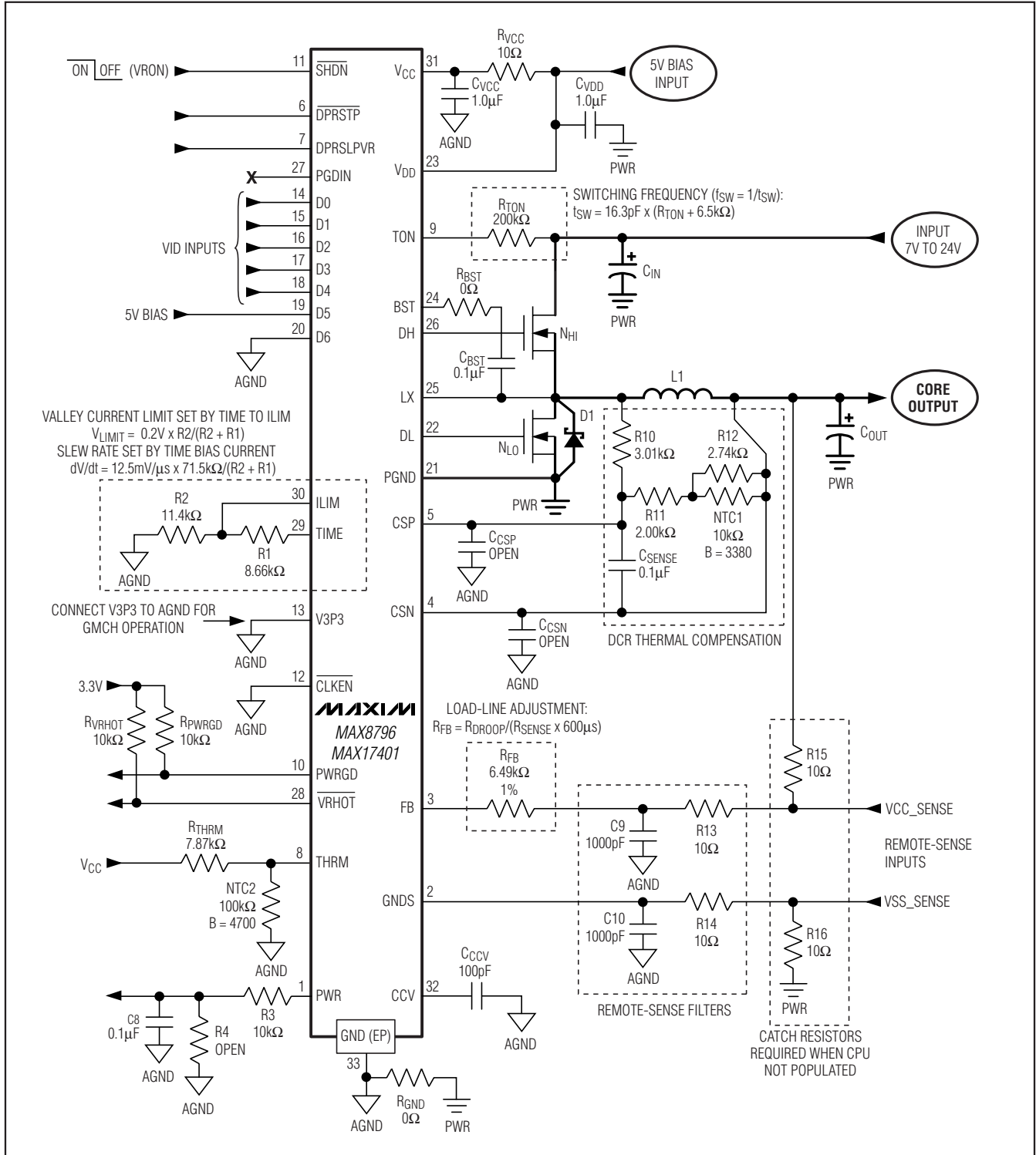
Figure 14. MAX8796/MAX17401 GMCH Standard Application Circuit
