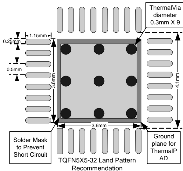
Figure 5. TQFN5X5-32 Land Pattern Recommendation
