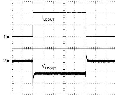
LDO Load Transient
