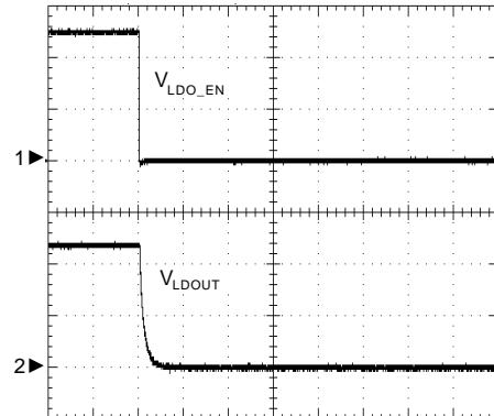
LDO Disable
