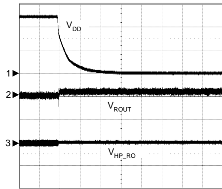
Power Off
