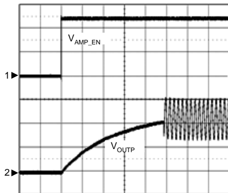
Speaker Enable
