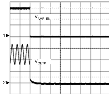
Speaker Disable
