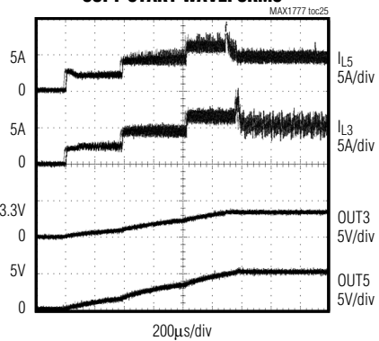
SOFT-START WAVEFORMS
